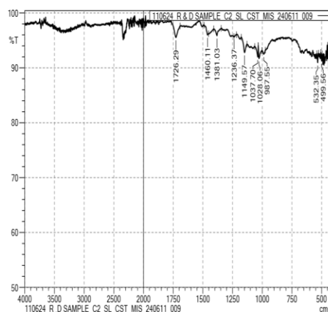
Figure 3: FTIR analysis with 0.35 % AIBN+ (Acrylate, Azoisobutyronitrile, Methanol) + Pinewood
