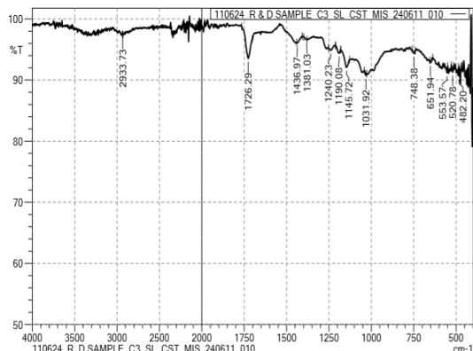
Figure 4: FTIR analysis with 0.50 % AIBN+ (Acrylate, Azoisobutyronitrile, Methanol) + Pinewood
