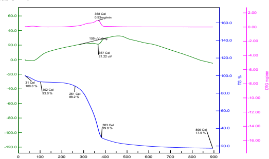
Figure 6: DTA and TGA analysis of Pinewood
