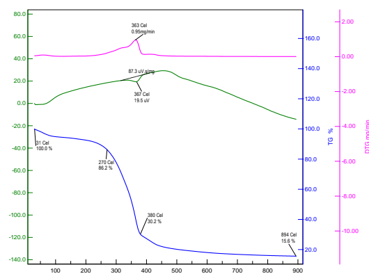
Figure 7: DTA and TGA analysis of Pinewood with 0.25 % AIBN+ (Acrylate, Azoisobutyronitrile, Methanol)
