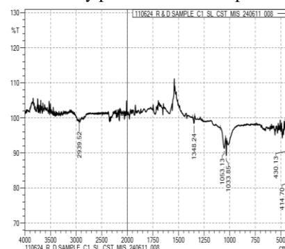
Figure 2: FTIR analysis with 0.25 % AIBN+ (Acrylate, Azoisobutyronitrile, Methanol) + Pinewood
