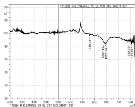
Figure 1: FTIR analysis of Pinewood
