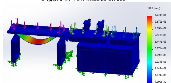
Figure 10. Displacement results
