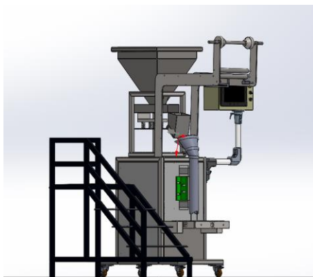
Figure 2. Grains packaging machine
