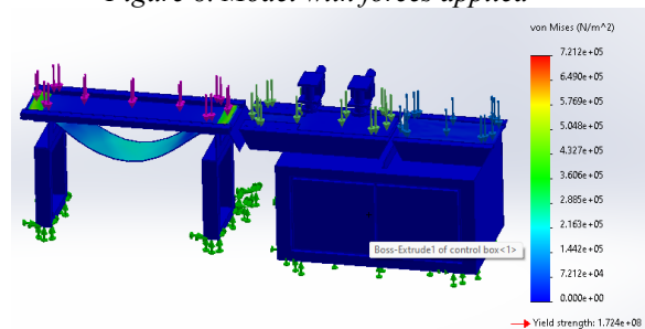
Figure 9. Von mises stress
