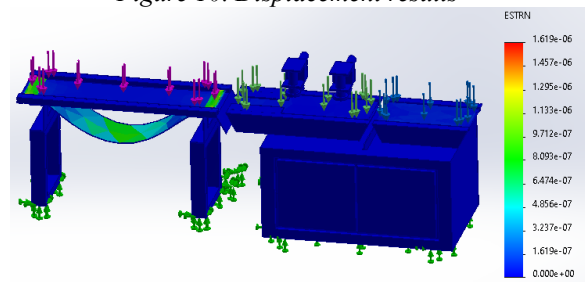
Figure 11. Strain analysis
