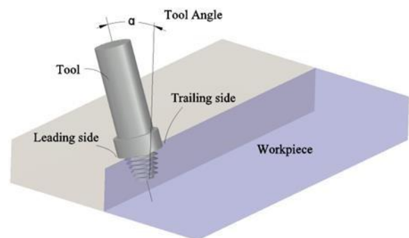
Fig. 6 Tool tilt angle (3-Dimension)
