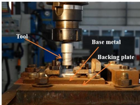
Fig. 1 Photograph showing the elements of FSW process
