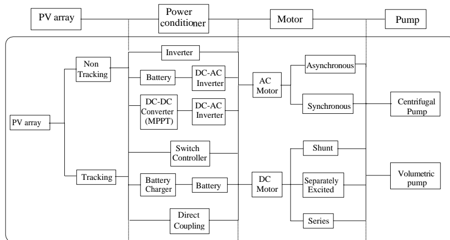
Fig (4) : Components of typical solar pump system
