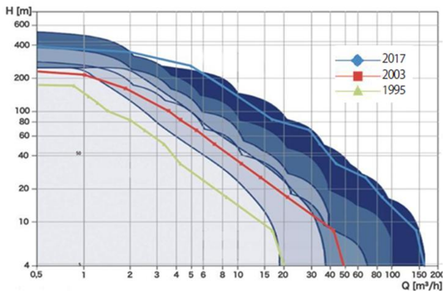
Fig (1) :Solar driven pump development
