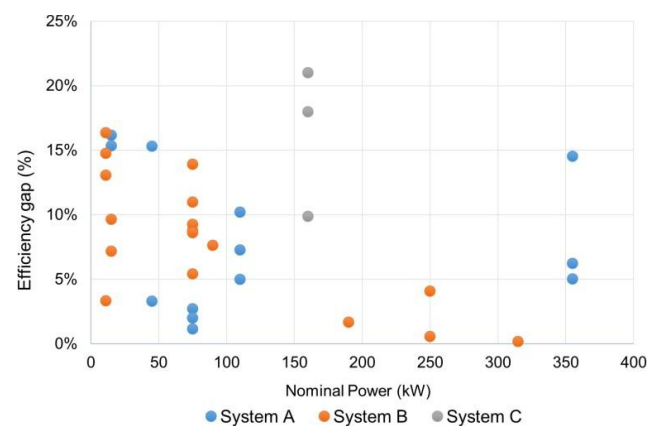
Fig 4 : Efficiency reduction and nominal power relation
