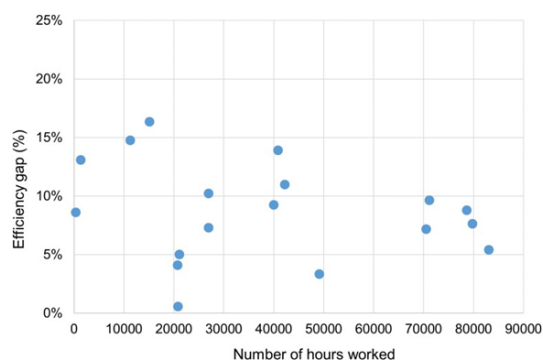
Fig 5 : Relation between Running hours and Efficiency reduction
