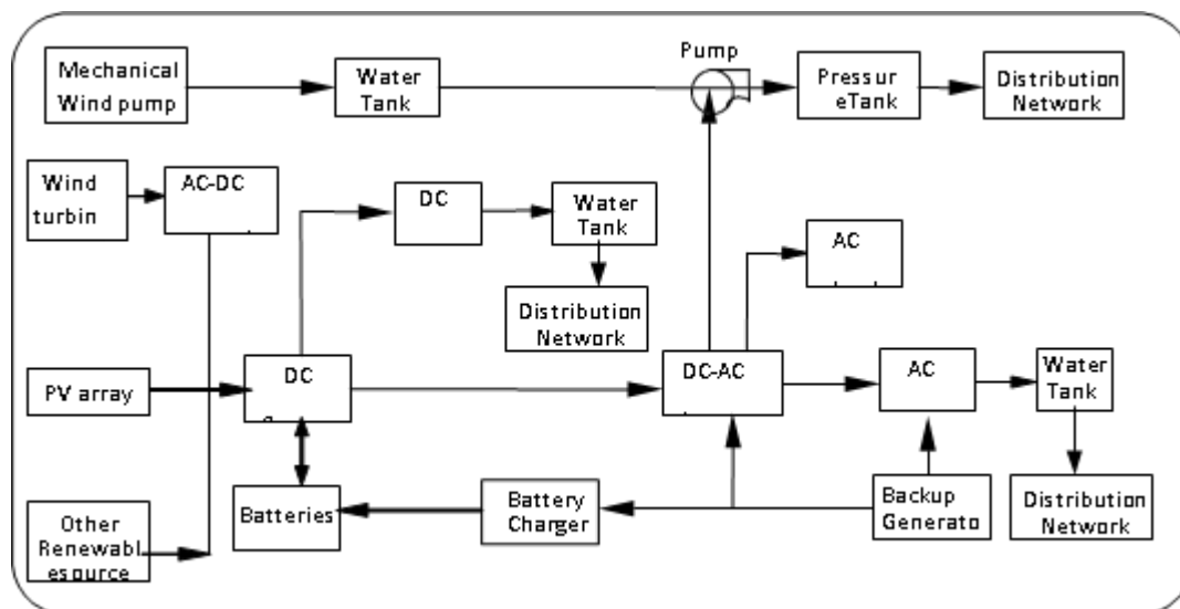
Fig (5) :Hybrid power system with backup generator
