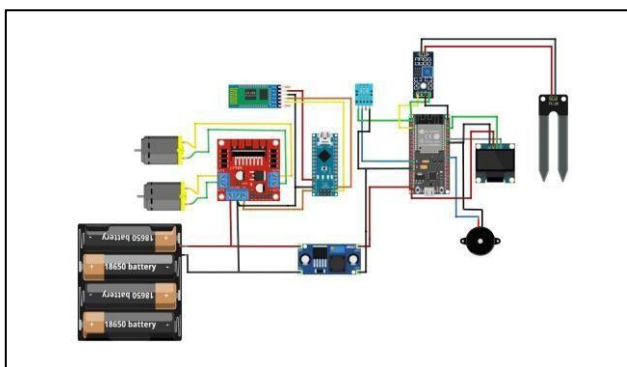
Figure-2 .Circuit Diagram Agriculture Monitoring System
