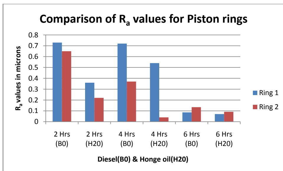
Figure 5 Comparison of R_a values for piston rings (B0 and H20)
