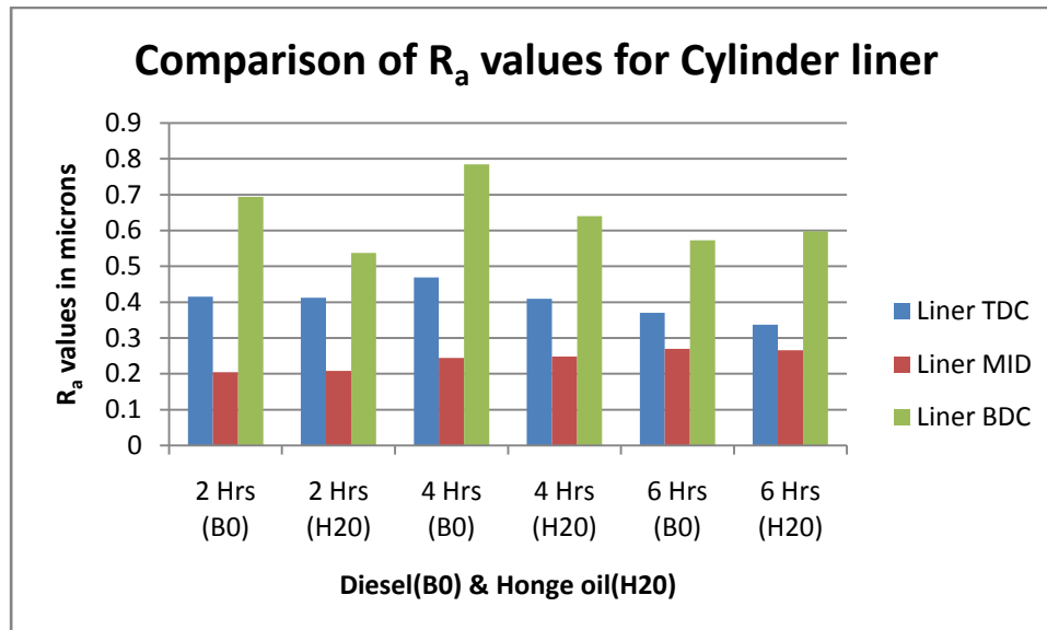
Fig. 3. Comparison of R a values for Cylinder Liner
