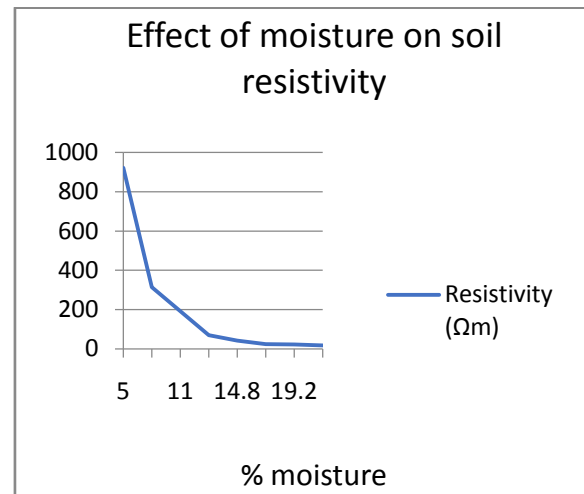
Figure 5: Effect of moisture content on soil resistivity
