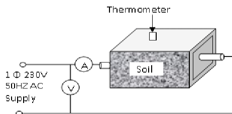
Figure 1: Soil resistivity measurements by sampling method.
