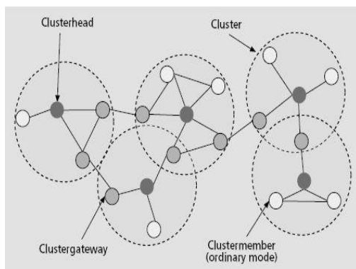
Figure 1.2 Clustered Networks
