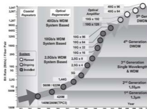
Fig.3. Generations of Fiber Optics Communication [8]
