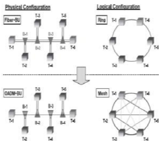
Fig.5. Optical Network Configurations [8]
