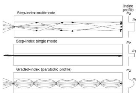
Fig.2. Optical Fiber Modes [6]
