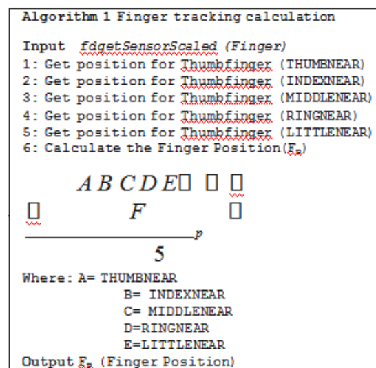
Figure 17. Pseudocode for finger position tracking
