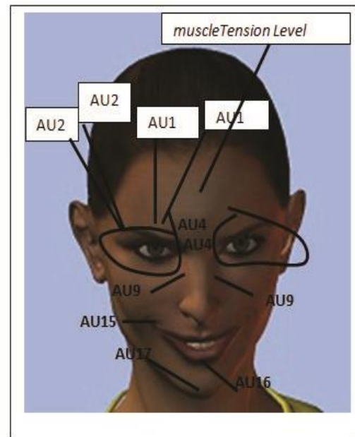
Figure 11. FACS regions
