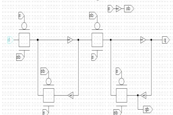
Fig 3. Circuit diagram of D flipflop using TG
