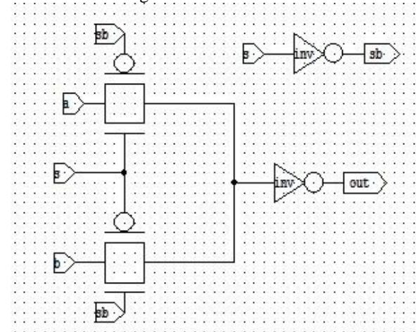
Fig 4. Circuit diagram for 2 to 1 multiplexer using TG
