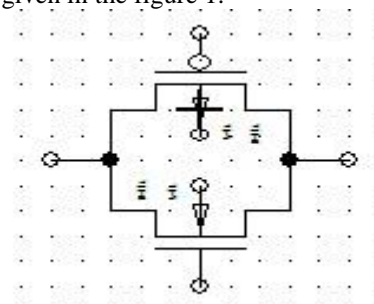
Figure 1. A simple transmission gate
