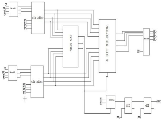
Fig 6. Block diagram of viterbi decoder
