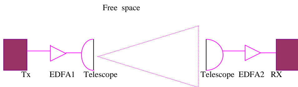
Fig. 1 Schematic diagram of a typical free-space optical system.
