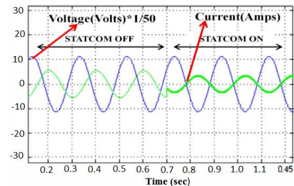
Fig.8. Instantaneous Value of grid Voltage and current for one phase.
