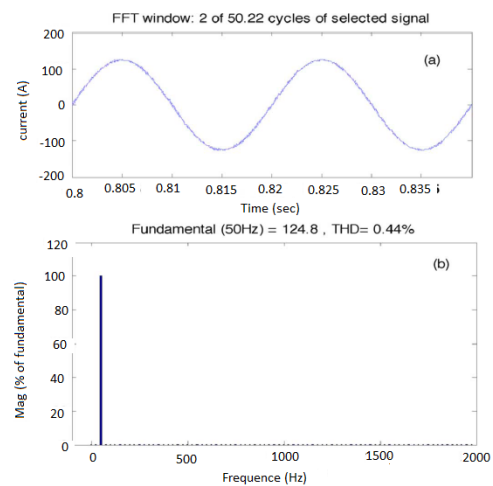
Fig.14. (a) Source Current. (b) FFT of source current.
