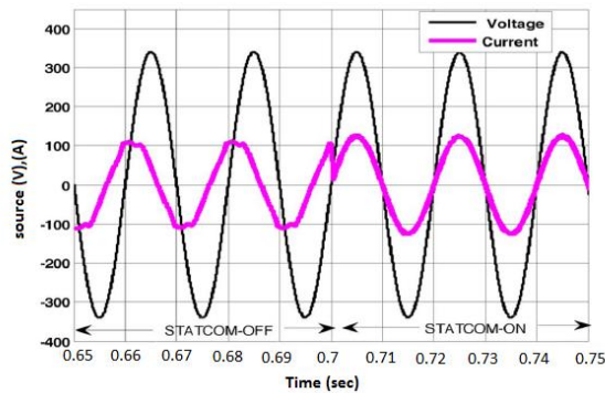
Fig 10. Supply Voltage and Current at PCC.
