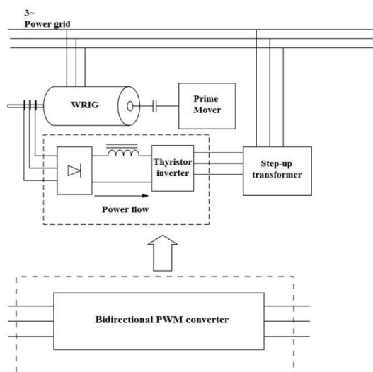
Fig 1: Doubly-fed induction generation system power flows.
