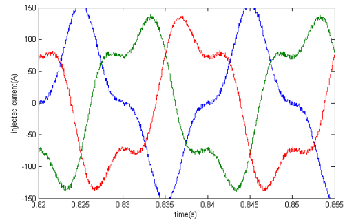
Fig 12.Three phase injected inverter current
