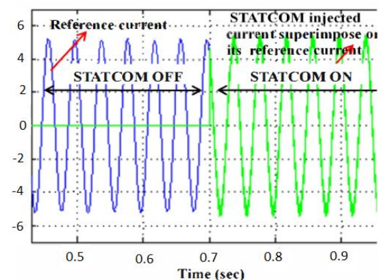
Fig.6. STATCOM injected current superimposed on its reference current.
