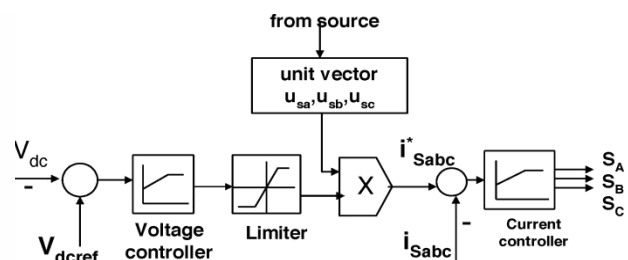
Fig. 4. Control system scheme
