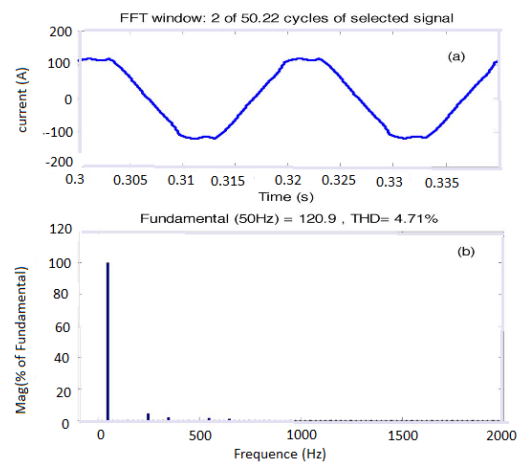
Fig.13. (a) Source Current. (b) FFT of source current.
