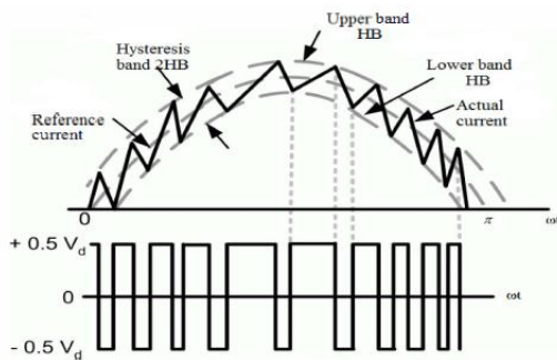
Fig 5: Hysteresis current modulation.
