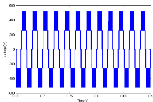
Fig.11.Output Waveform of inverter.
