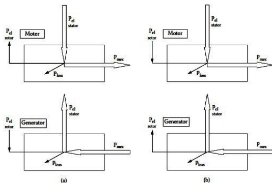
Fig 2: Operation modes of DFIG with bidirectional pulse-width modulator (PWM) converter (in the rotor): (a) S < 0 and (b) S > 0 .
