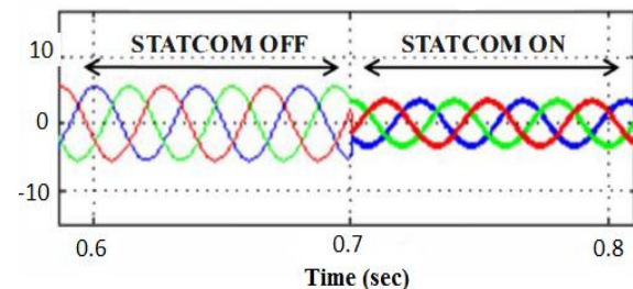
Fig.7. source current
