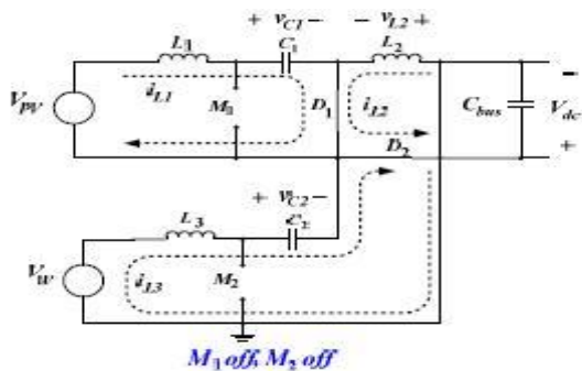
Figure 5: M1 off, M2 off
