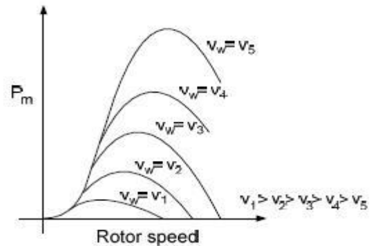
Figure 7: Power Curves for a typical wind turbine
