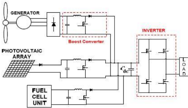
Figure 1: Hybrid System with multi-connected boost converter
