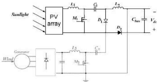
Figure 4: M1 off, M2 on
