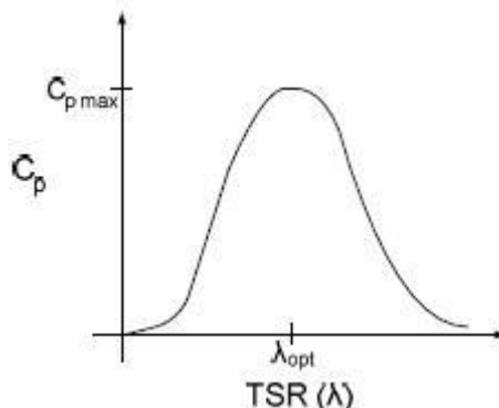
Figure 6: Power Coefficient Curve for a typical wind turbine
