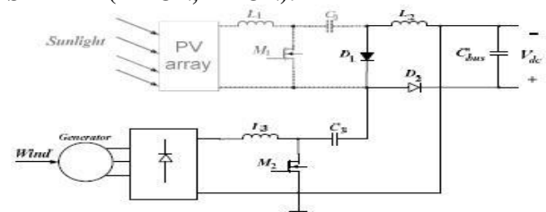
Figure 3: M1 on, M2 on
