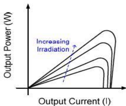
Figure 10: Output Power Vs Output Current
