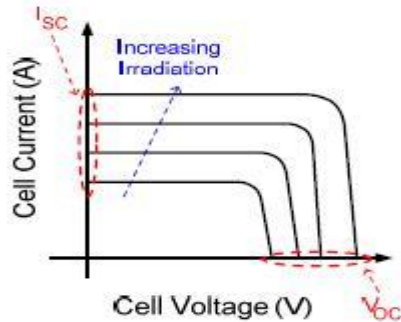
Figure 9: Cell Current Vs Cell Voltage
