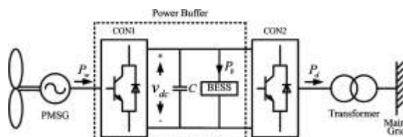
Fig-1: Block diagram of Wind Energy System with BESS
