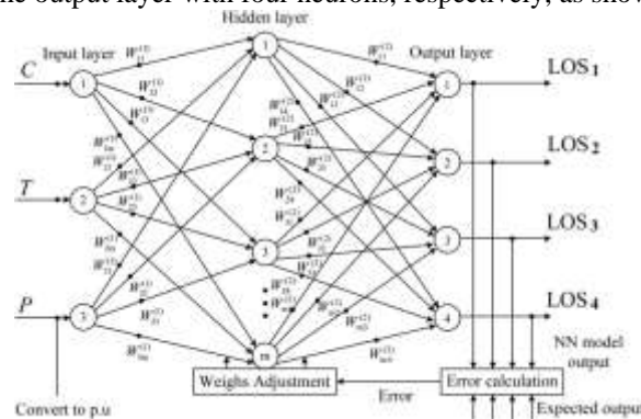
Fig. 3 Structure of the ANN
