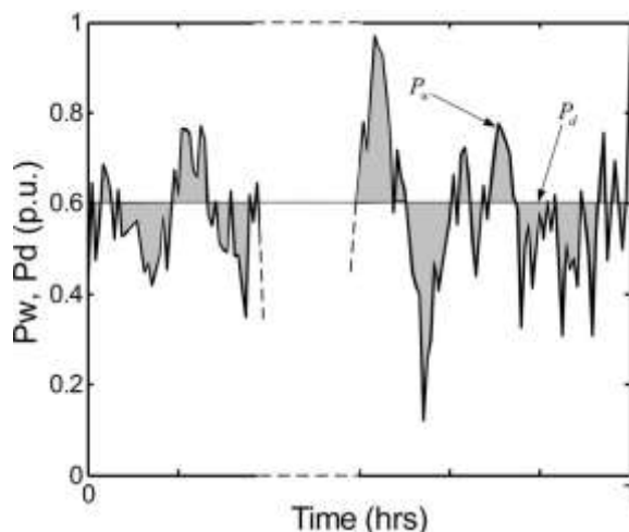
Fig-2: Typical wind power profile
