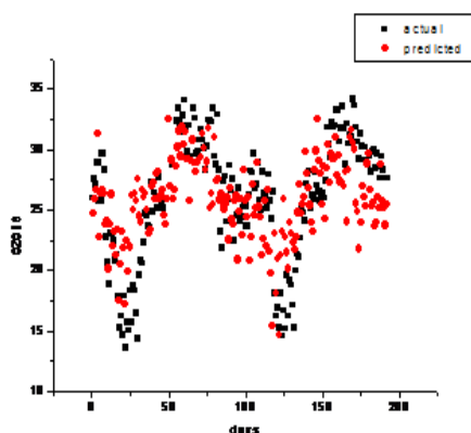
Fig.5.4. Actual and predicted values of ozone
