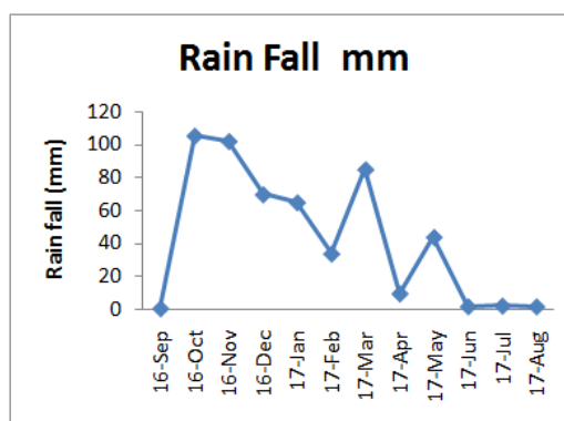
Fig.2 Monthly average variations of relative humidity, wind speed, maximum temperature, minimum temperature and rainfall
