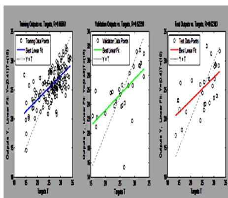
Fig. 5.3. Model Results
