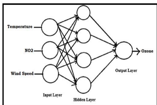
Fig. 5.2 Proposed neural network model for ozone
