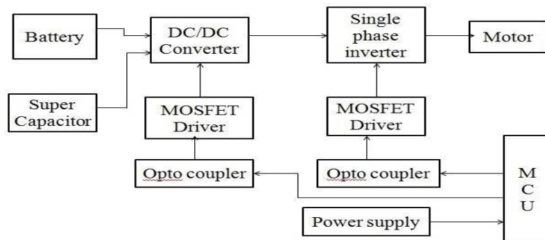
Figure 1: Hybrid energy storage system for electric vehicle 2
