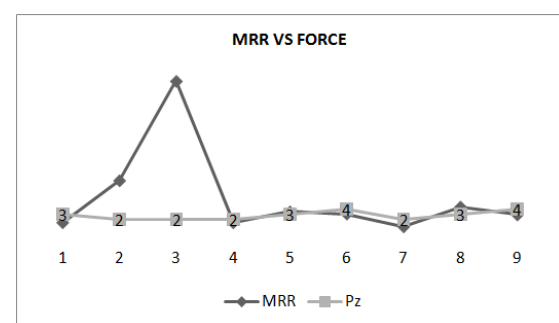
Fig.-5.16: Material removal rate vs Cutting force ( P_z )
