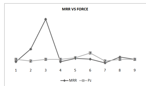
Fig.-5.20: Material removal rate vs Cutting force ( P_z )
