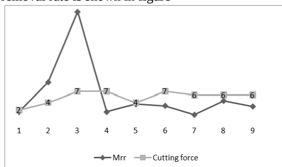
Fig.-5.2: Material removal rate vs Cutting force (Pz)
