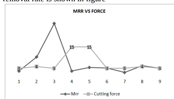
Fig.-5.8: Material removal rate vs Cutting force ( P_z )
