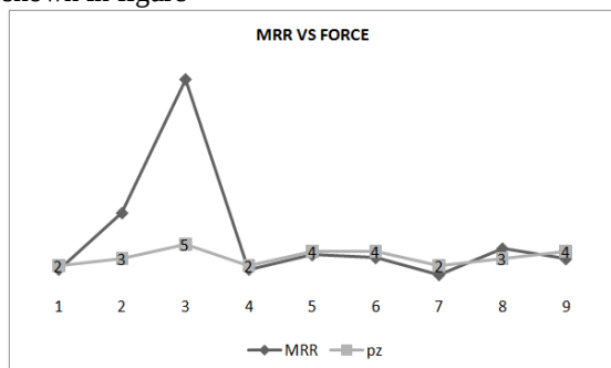
Fig.-5.14: Material removal rate vs Cutting force ( P_z )
