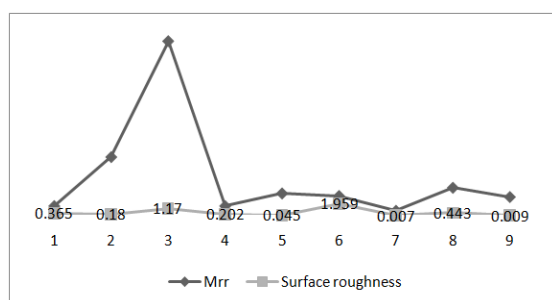
Fig.-6.1: Material removal rate vs surface roughness
