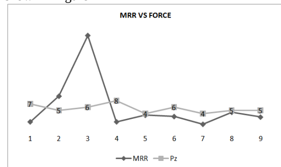
Fig.-5.12: Material removal rate vs Cutting force ( P_z )
