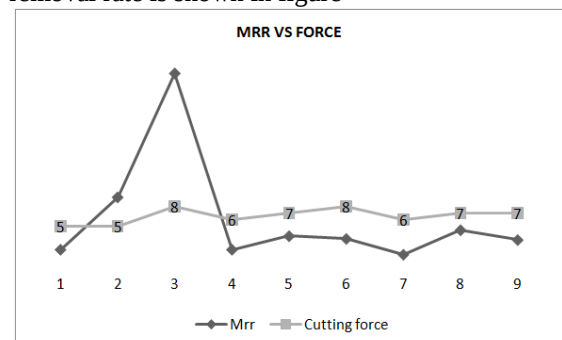
Fig.-5.4: Material removal rate vs Cutting force (Pz)
