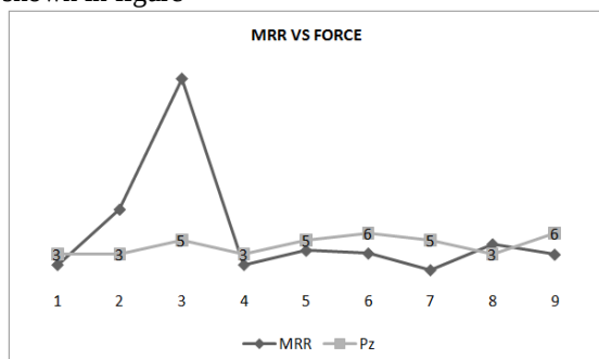
Fig.-5.18: Material removal rate vs Cutting force ( P_z )
