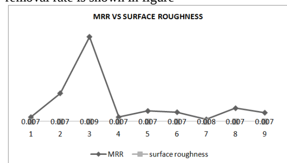
Fig.-5.19: Material removal rate vs Surface roughness
