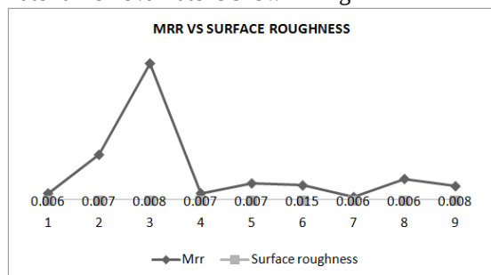
Fig.-5.5: Material removal rate vs surface roughness
