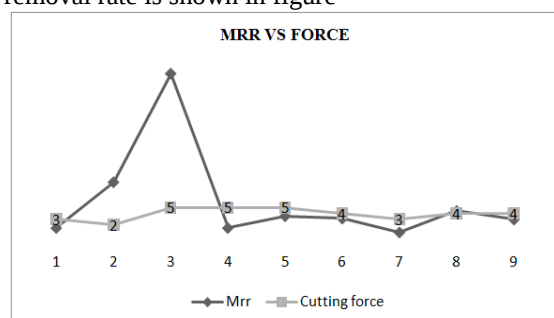
Fig.-5.10: Material removal rate vs Cutting force ( P_z )
