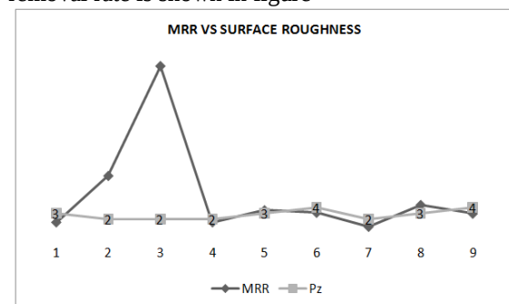
Fig.-5.15: Material removal rate vs Surface roughness
