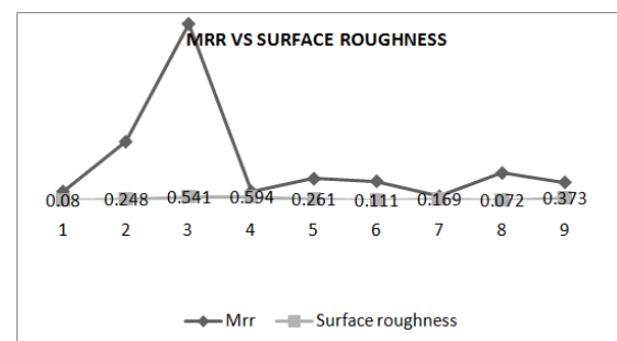
Fig.-5.3: Material removal rate vs surface roughness
