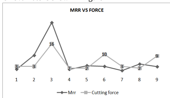
Fig.-5.6: Material removal rate vs Cutting force ( P_z )
