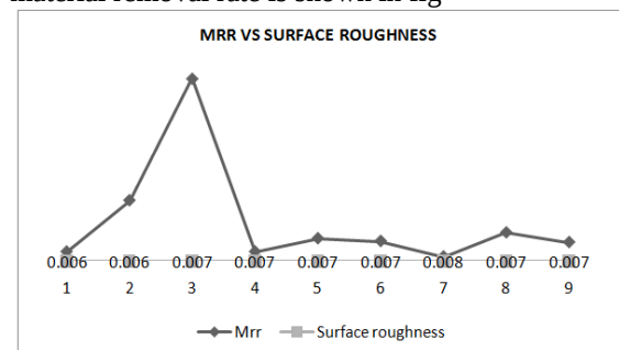
Fig.-5.7: Material removal rate vs Surface roughness
