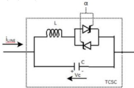
Fig 3: Basic TCSC module
