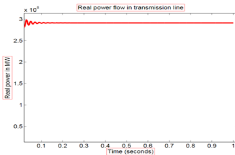
Fig 11: Real power flow in transmission line for uncompensated system
