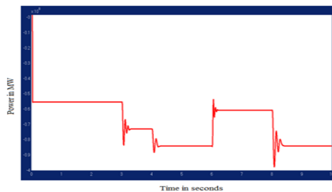
Fig 13: Real Power Flow Control in transmission line using TCSC with FLC from area2 to area1
