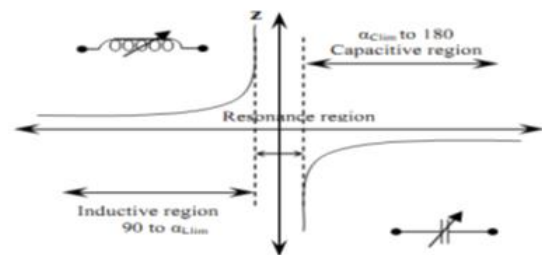
Fig 4: Characteristics of TCSC
