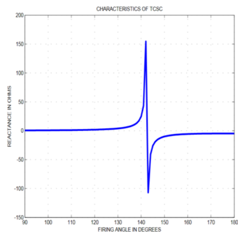
Fig 5: Characteristics of TCSC
