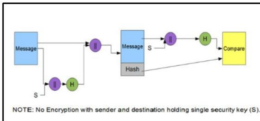
Fig:Basic hash function
