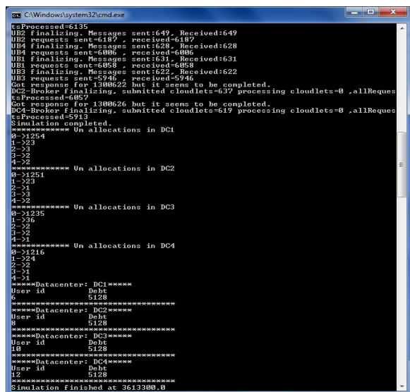
Figure 6. Assigned VM in Data Centers
