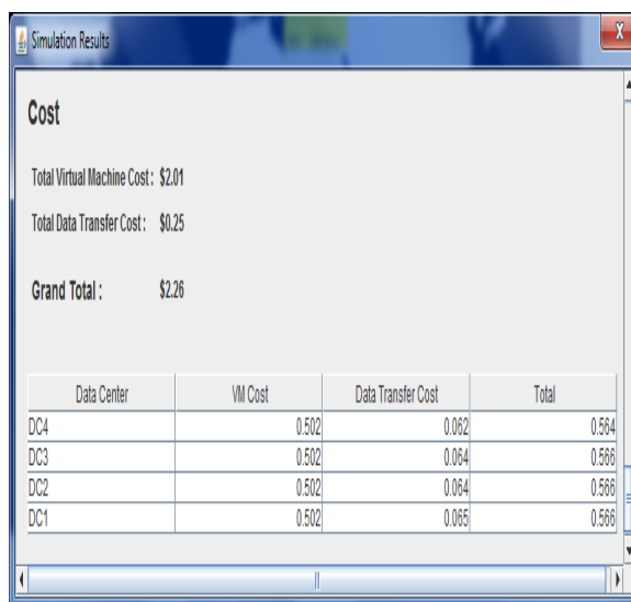
Figure 4. Cost of Data Center with Data Transfer Cost
