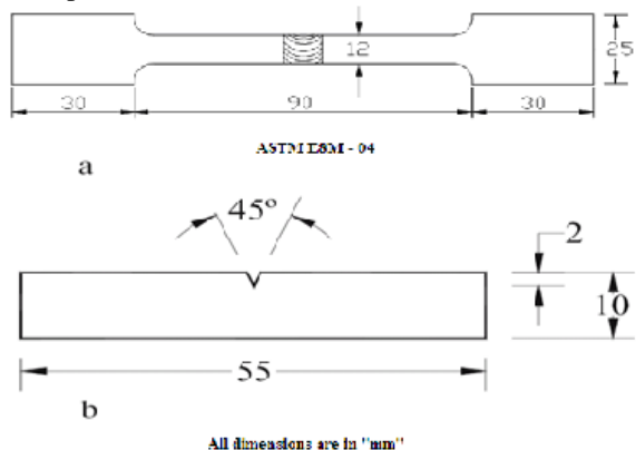
Schematic diagram of a tensile and b impact specimen
