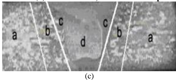
Fig. 3-Different regions of FSW joint: (a) unaffected base metal; (b) heat affected zone (HAZ); (c) thermo-mechanically affected zone (TMAZ); (d) friction stir processed (FSP) zone.
