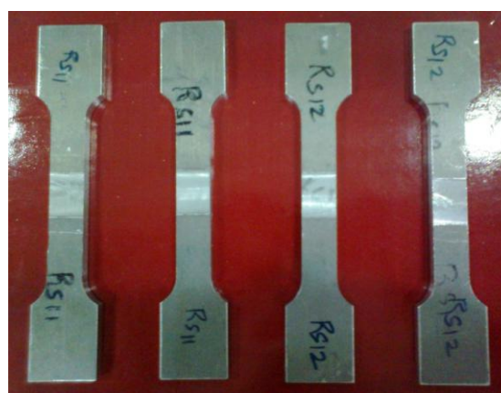
Fig. 7. Tensile test specimens of Friction Stir Welded joints of A7075 before testing.
