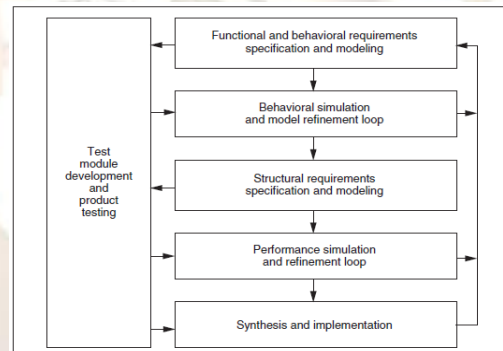
Figure 1. Abstract design flow in model-based codesign.
