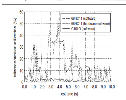
Figure 5. Microcontroller utilization over time for scenario B.
